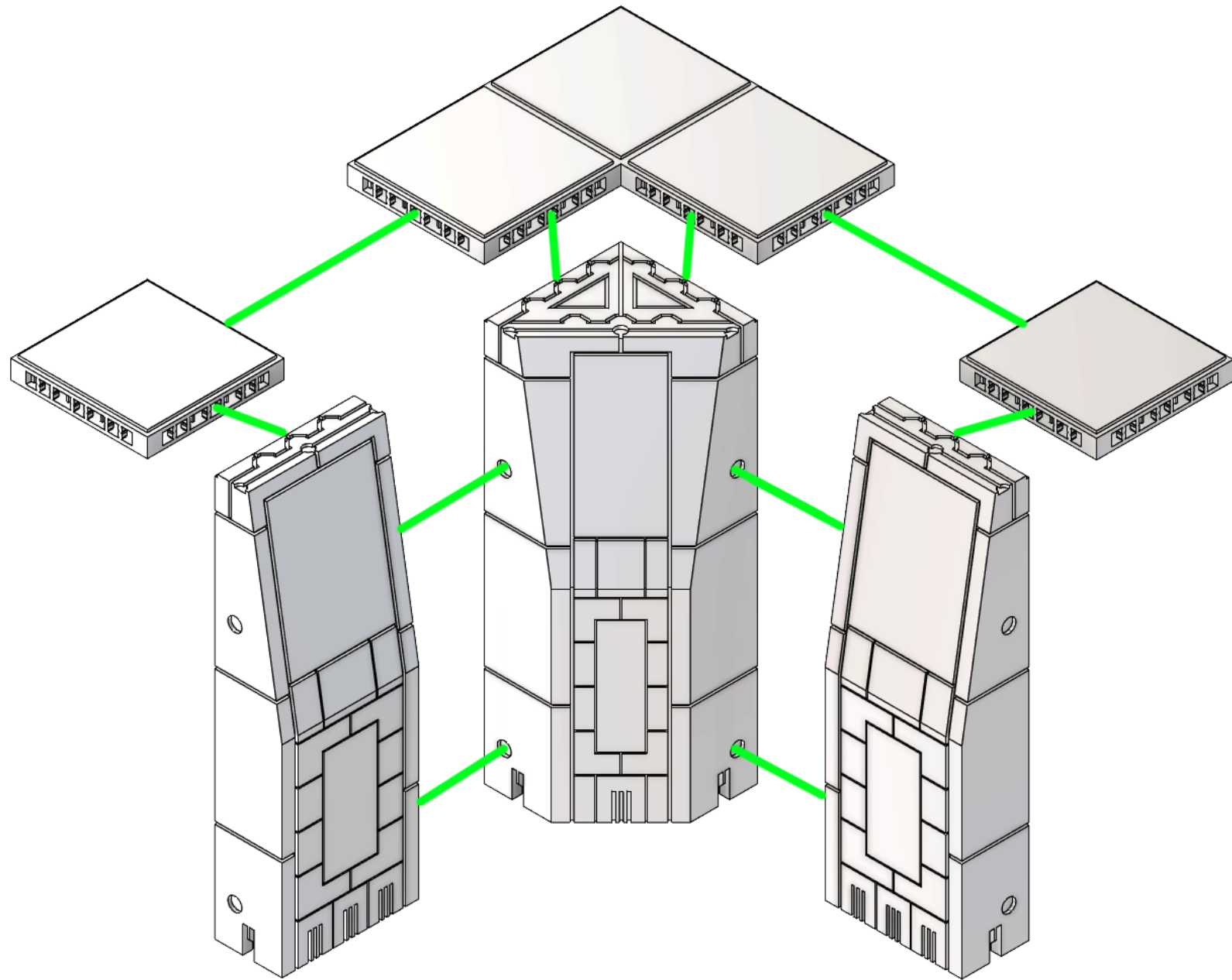
INSIDE CORNER ASSEMBLY
