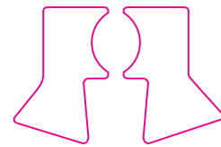
L/R TOP OF SEATSTAY BEFORE WELD
