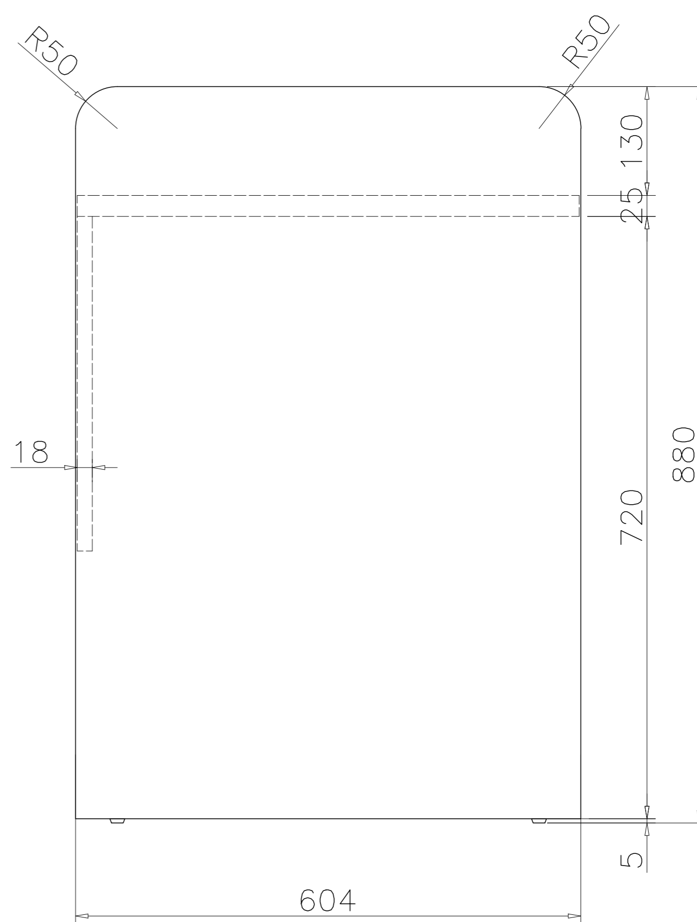
SIDE VIEW
