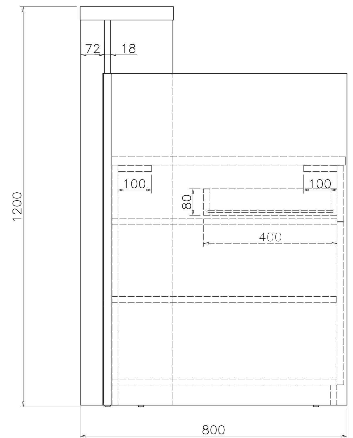
SIDE VIEW
