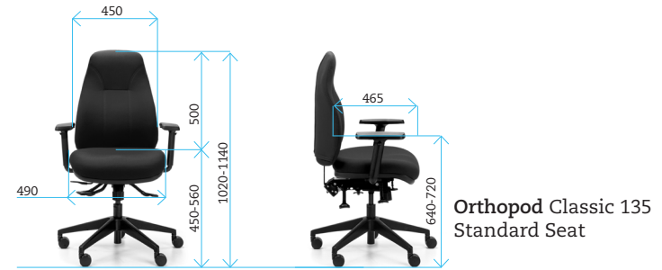
compressed seat height as per AFRDI measurements.
