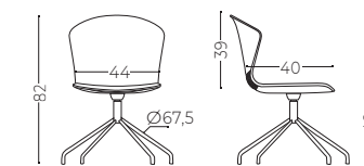
4 Spoke base with pads chair Silla base 4 brazos tapones - Giratoria
