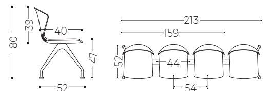
Beam seating Bancada
