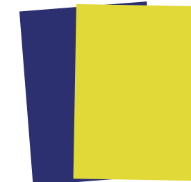
HDPE Panel Sheet Thickness: 1/4", 1/2", or 3/4" Size Part No. 1/4" x 48" x 96" PS-25 1/2" x 60" x 120" PS-50 3/4" x 60" x 120" PS-750
