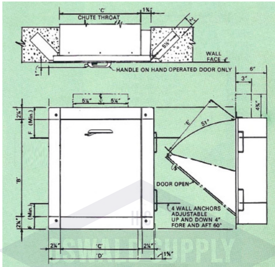
Wilkinson Style "Signature Series" Stainless Steel Trash Chute Door DIMENSION CHART
