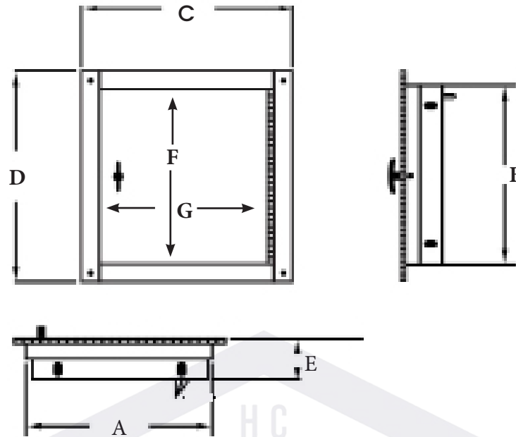
UNIVERSAL STAINLESS STEEL LINEN CHUTE DOOR DIMENSION CHART (WITH CONNECTED TRIM – STANDARD WIDTH 2.13”)
