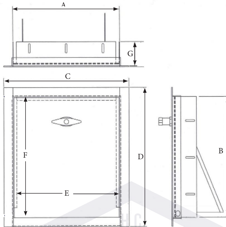
UNIVERSAL STAINLESS STEEL TRASH CHUTE DOOR DIMENSION CHART
