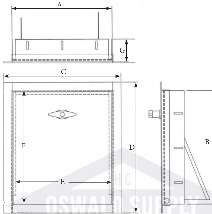
UNIVERSAL STAINLESS STEEL TRASH CHUTE DOOR SKU: HRX09 DIMENSION CHART
