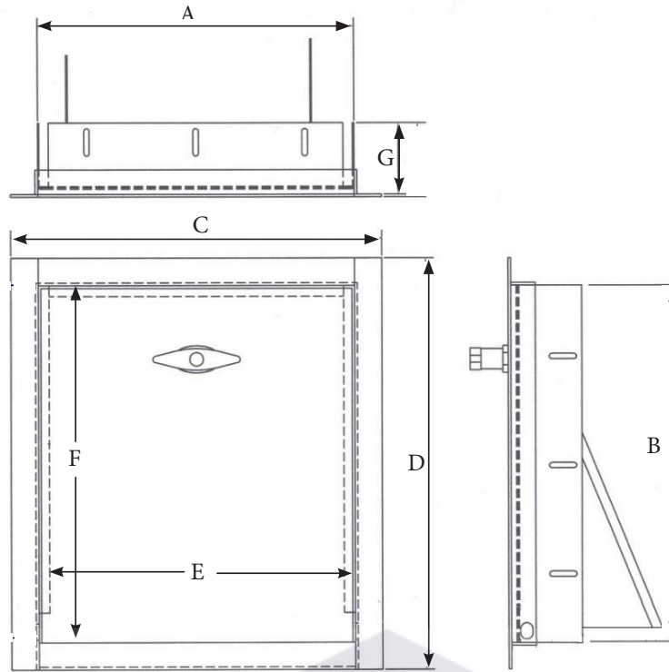
UNIVERSAL STAINLESS STEEL TRASH CHUTE DOOR SKU: HFX09 DIMENSION CHART
