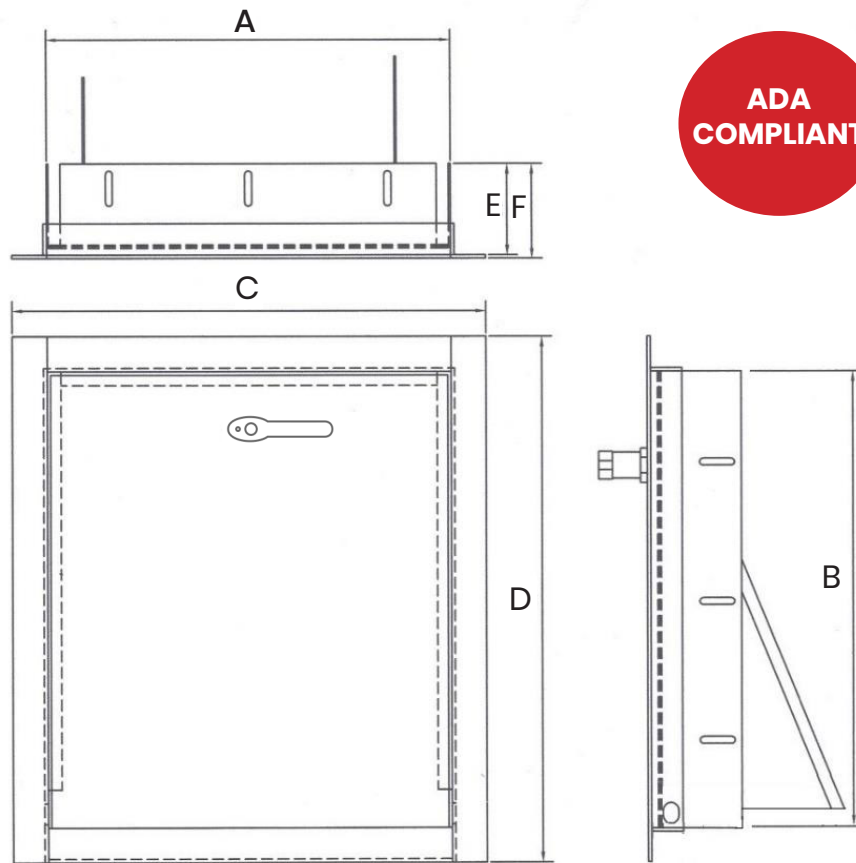
UNIVERSAL LARGE STAINLESS STEEL TRASH CHUTE DOOR SKU: HRX09ADA DIMENSION CHART (WITH CONNECTED TRIM – STANDARD WIDTH 2.25”)
