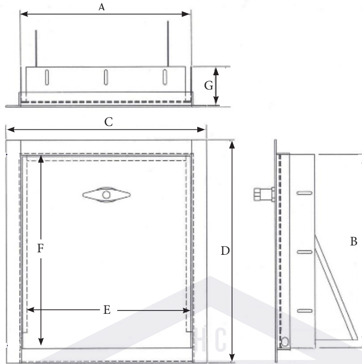
REPLACEMENT STAINLESS STEEL TRASH CHUTE DOOR DIMENSION CHART
