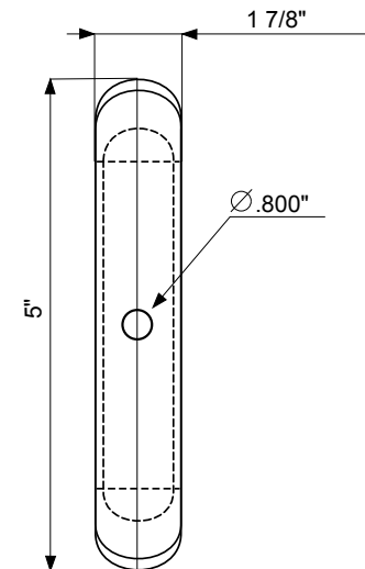
CRAB/YOKE TOP VIEW
