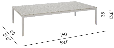
150x80 - coffee table 35h OST0004970
