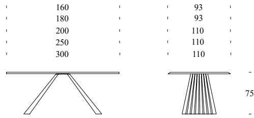
8011FL- fixed - wooden top
