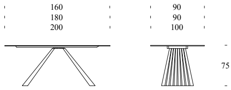
8011 - extendible - tempered glass / ceramic glass top
