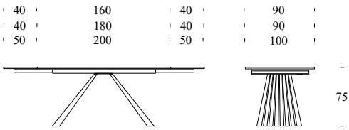
8011 - extendible - tempered glass / ceramic glass top
