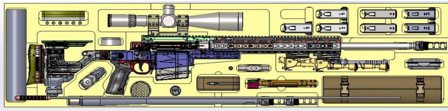
AI-29915-XX LAYOUT SHOWING DIFFERENT CONFIGURATIONS
