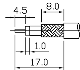
STRIPPING DIMENSION
