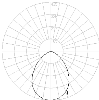
Luminous Intensity Distribution Diagram (cd)
