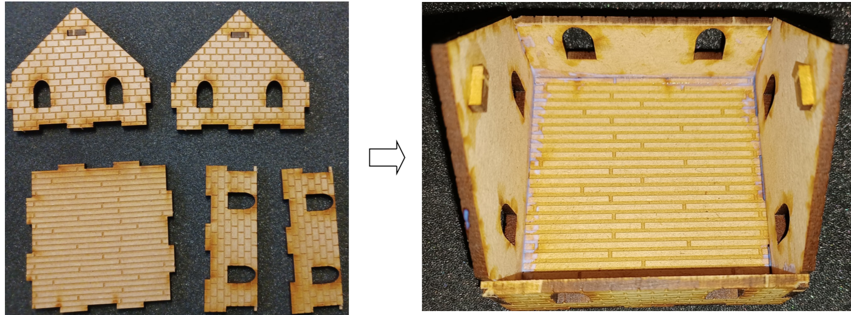
12: Glue shown pieces together for the 2nd floor of the Church Tower.
