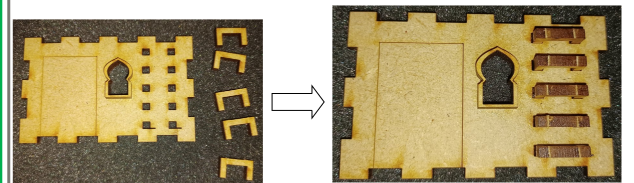
11: Glue stairs for roof onto wall piece.
