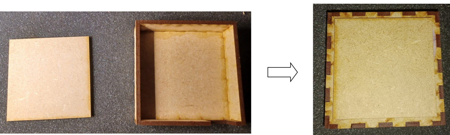
9: Glue shown piece onto bottom of the 1st floor roof. Make sure piece is centered.
