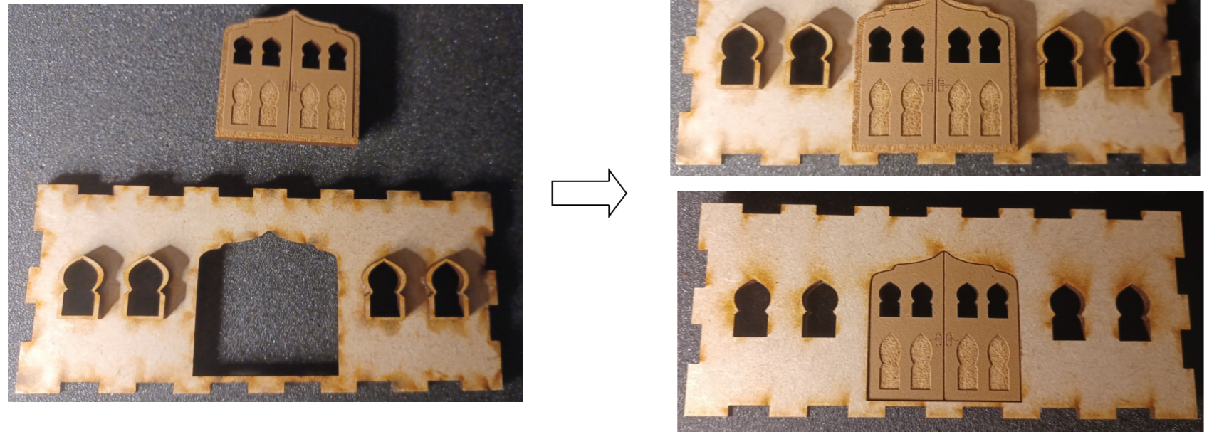
8: Glue shown piece onto bottom of the 1st floor. Make sure piece is centered.
