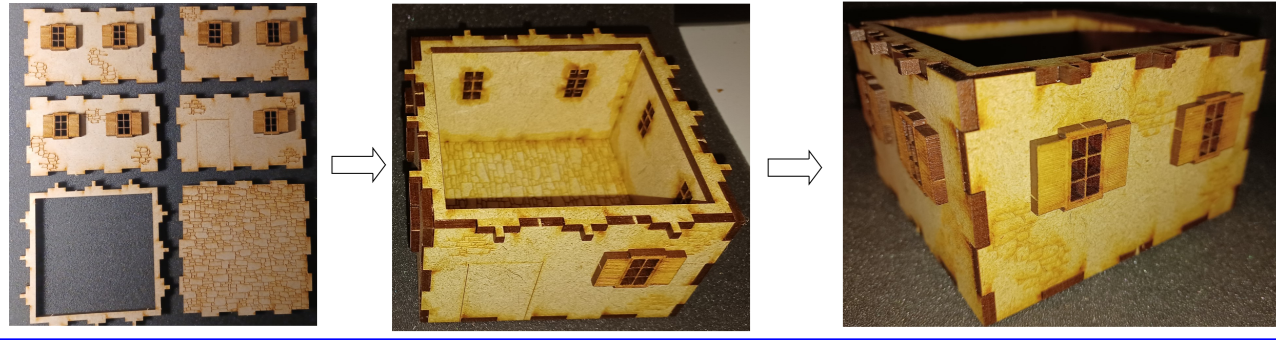
6: Glue together shown pieces for the ground floor. House 2
