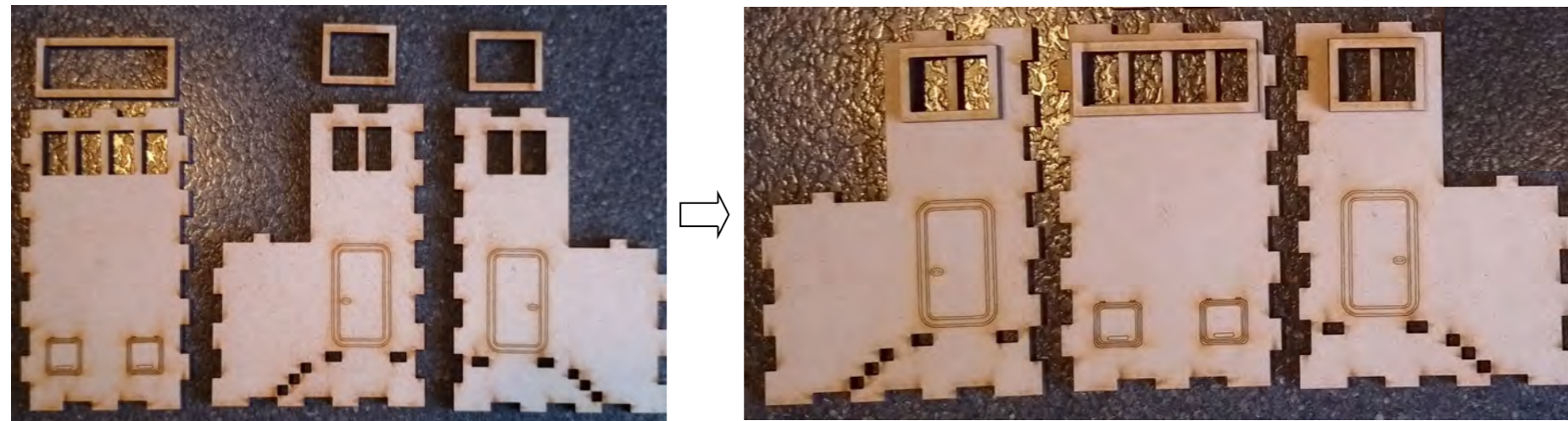
16: Glue window frames onto the bridge parts
