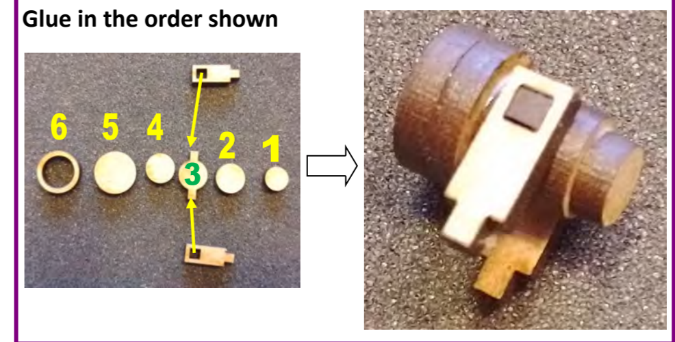
15: Glue together shown pieces for the search light.
