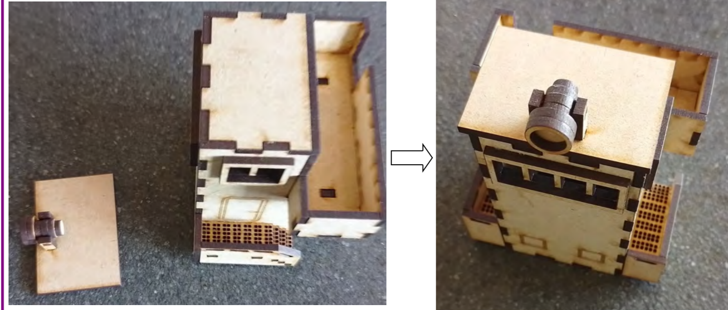
26: Glue the roof onto the Bridge.
