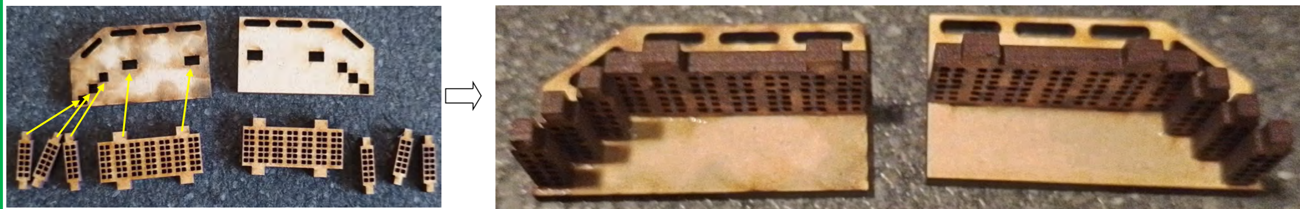
14: Glue together shown pieces for the two staircases to the bridge.
