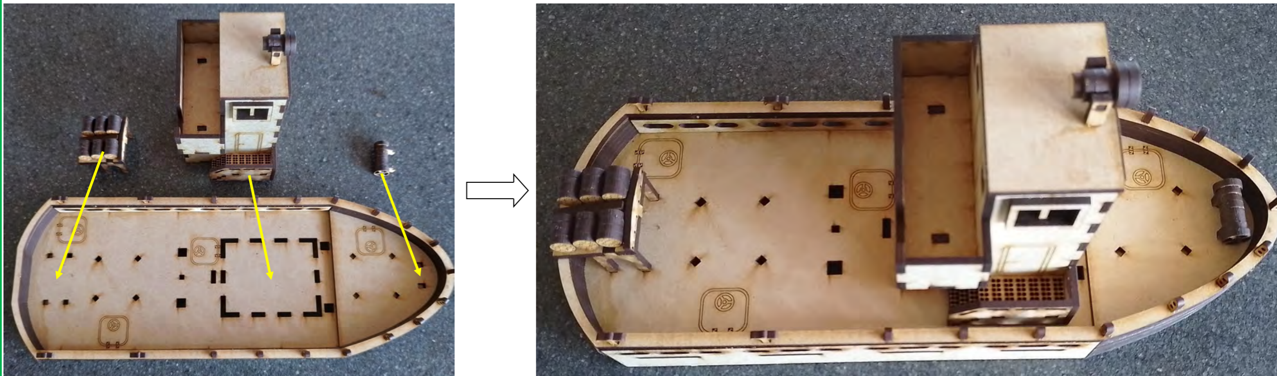
28: Glue the Bridge, cable hoist, and depth charges platform onto the ship's deck.
