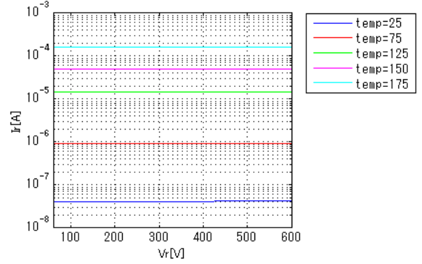
IrVr(Breakdown)
