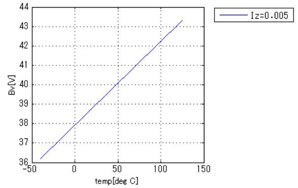
IrVr(Breakdown)
