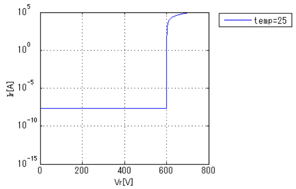
IrVr(Breakdown)
