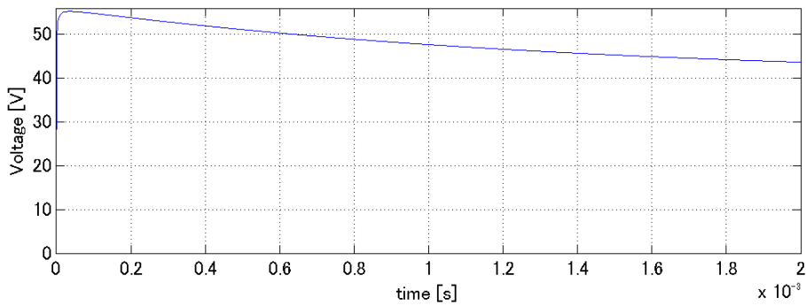
SurgeWaveform(Reverse Current 10/1000us)
