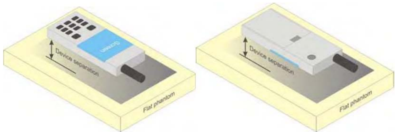
Figure 5 – Test positions for body-worn devices
