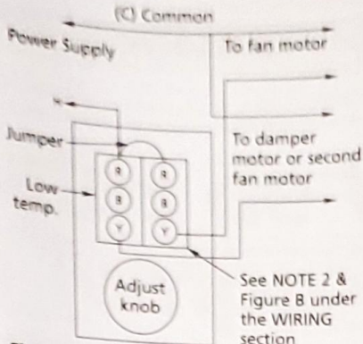
Figure 5 - Two-stage SPDT/SPDT Thermostats in Control of a Single-speed Ventilating Fan and Volume Increase Damper Motor
