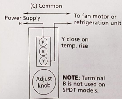
Figure 2 - Connection for a Typical Refrigeration, Ventilation or Cooling Control Circuit
