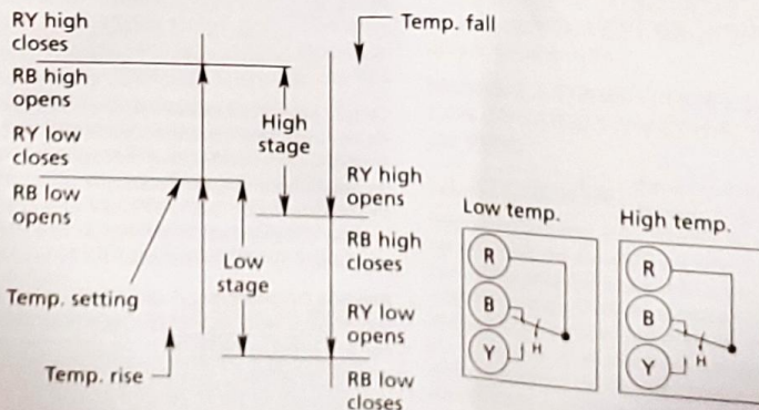
Figure 8 - Operational Sequence of Two-stage SPDT/SPDT Thermostats
