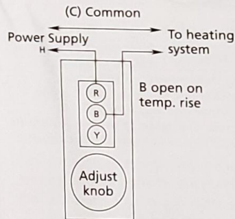
Figure 1 - Connection for a Typical Heating Control Circuit
