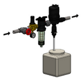
In-line installation
