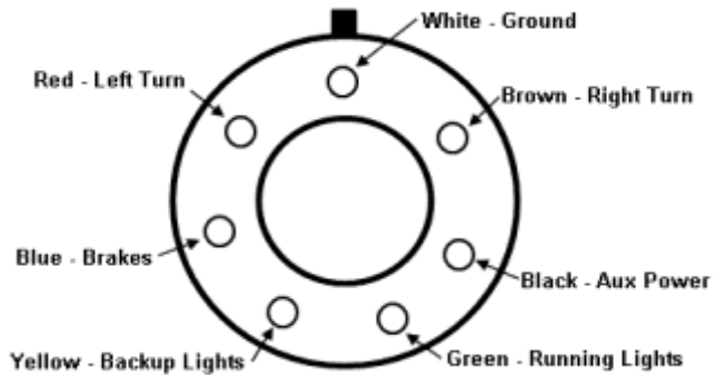
Figure 1 Looking into the Vehicle Socket (The trailer plug is exactly the opposite so they match when plugged together)
