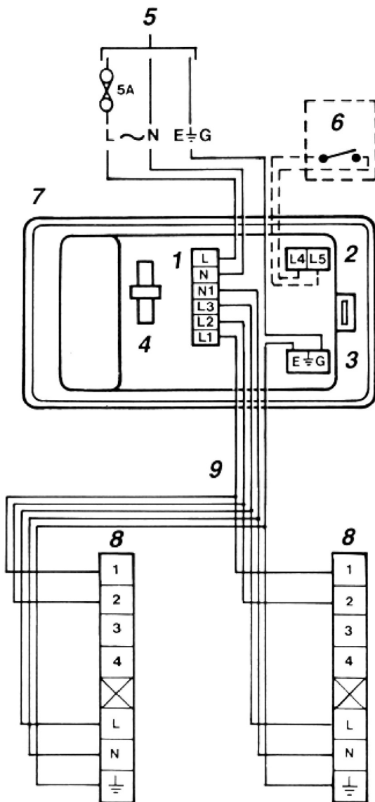
Current heat recovery ventilation unit terminal blocks as fitted to HR500 MKIII and HR500X units Refs 14101010B & 14101070
