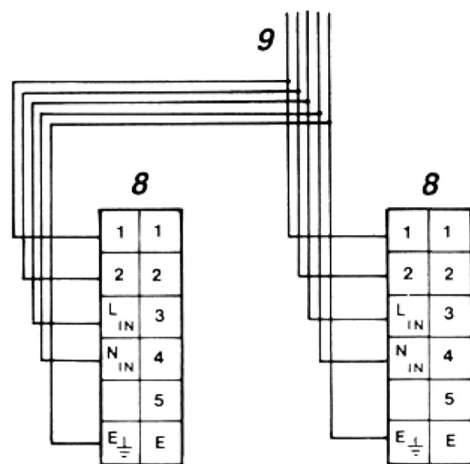
Earlier heat recovery ventilation unit terminal blocks as fitted to HR500 MKI and MKII units Refs 14101010 & 14101010A
