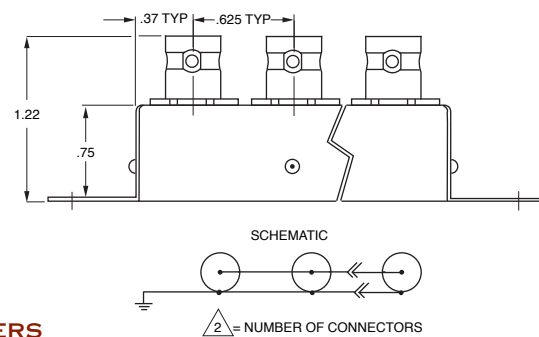
ADAPTERS MULTIPLE PARALLEL NETWORK 50Ω MPN- \triangle /BNC 50Ω MPN- \triangle /TNC Contact the factory for more information.
