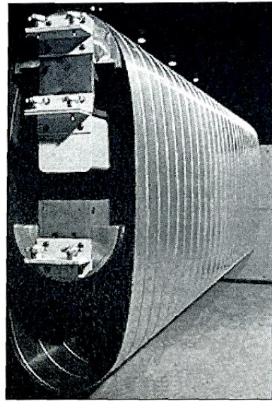
Finished flat oval duct after stretching
