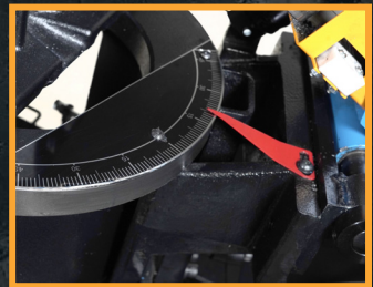
LARGE PROTRACTOR FOR ACCURATE AND FAST ANGLE CUTS
