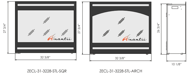
ZECL-31-3228-STL-SQR
