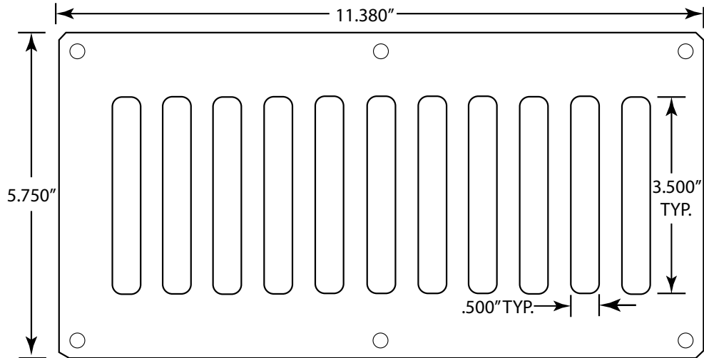
Fig. 1 Vent dimensions.
