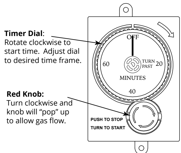
Fig. 4 E-Stop operation.
