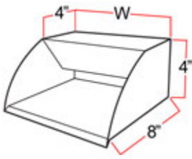
Radius Scupper
