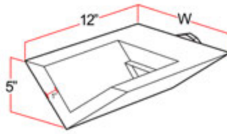
V-Shaped Scupper
