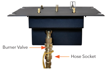
Photo A2: Quick Connect Properly Connected to Burner Box
