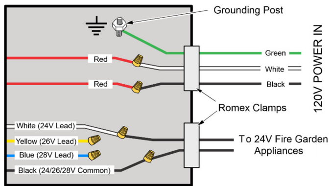
Transformer Junction Box
