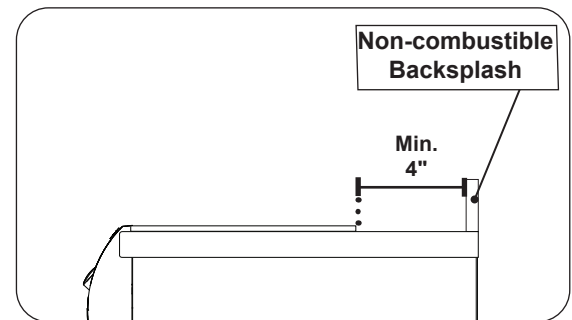
Fig. 16-4 Backsplash clearance
