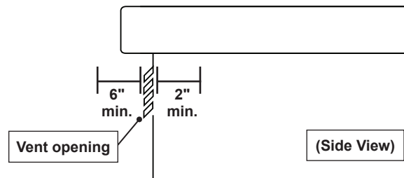
Fig. 11-2 Vent openings clearance
