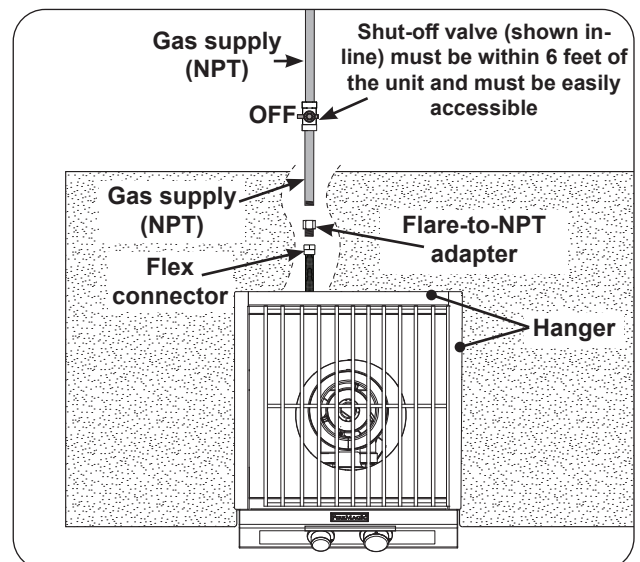
Fig. 25-2 Household L.P. & nat. gas diagram
