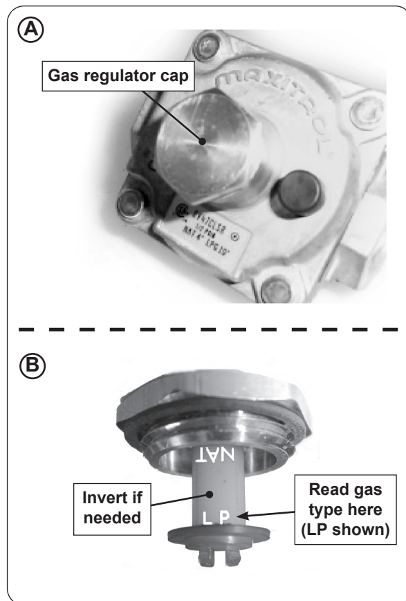
Fig. 38-1 Convert regulator
