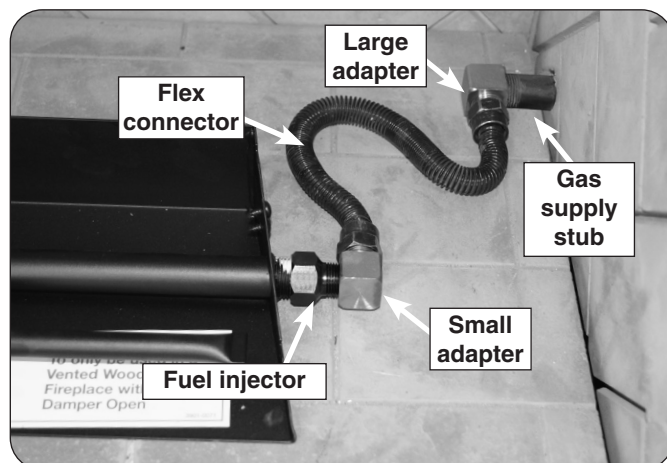
Fig. 9-1 Connect gas supply
