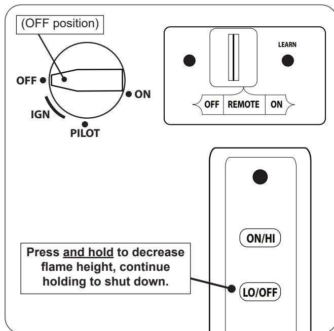
Fig. 43-2 Remote shut down
