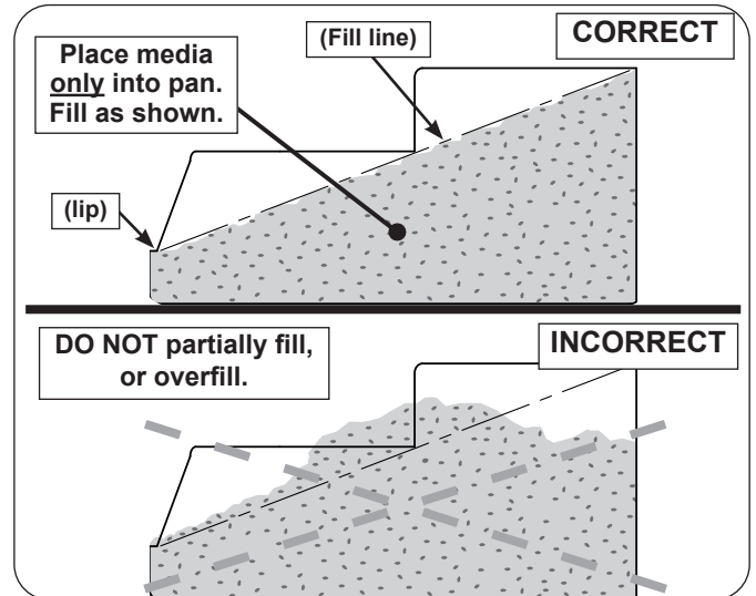
Fig. 19-2 Correct / Incorrect media placement
