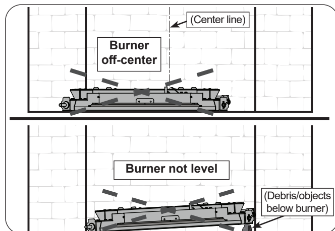
Fig. 14-3 INCORRECT burner pan placement
