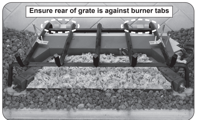
Fig. 20-3 Place grate
