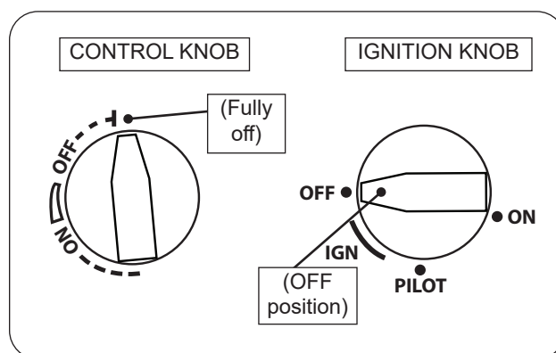
Fig. 42-2 Manual shut down
