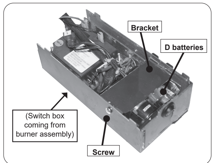
Fig. 15-3 Install burner system batteries
