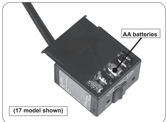
Fig. 15-2 Install remote receiver batteries
