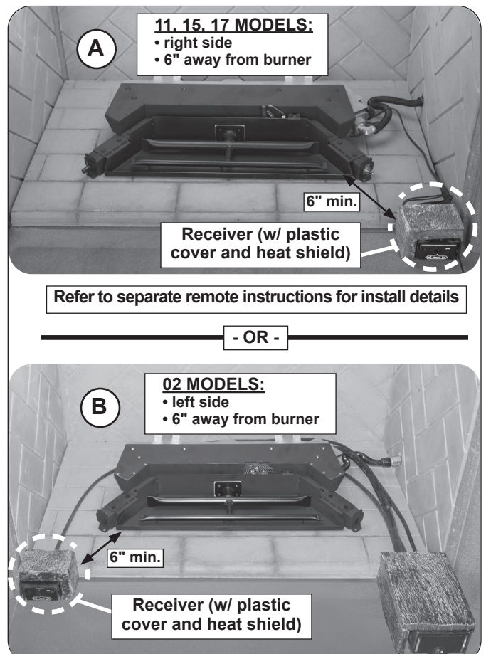
Fig. 16-2 Install remote receiver (if equipped)
