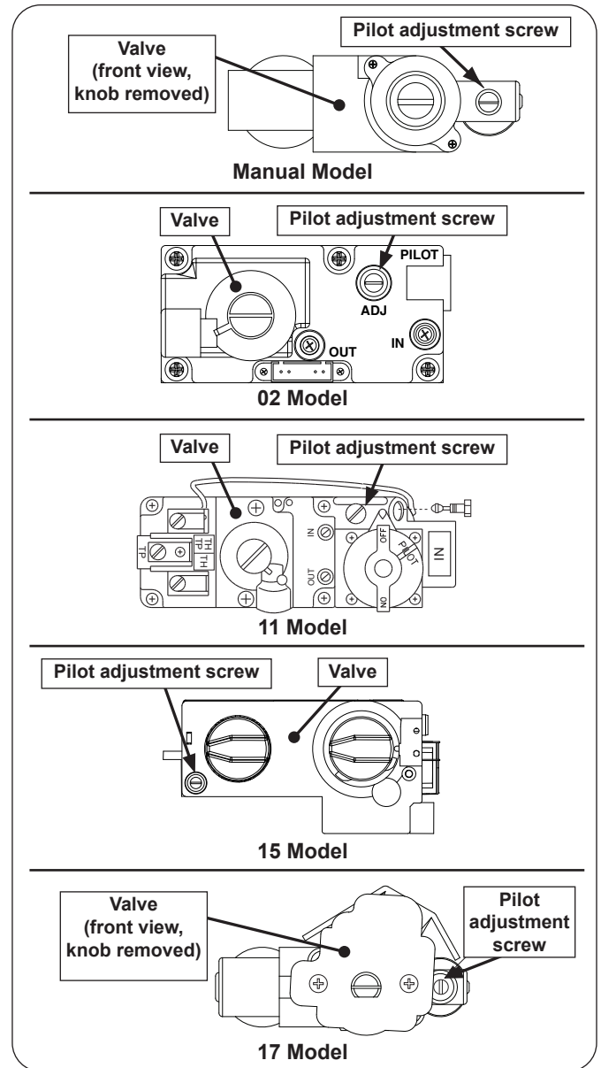
Fig. 17-2 Pilot adjustment detail (if needed)
