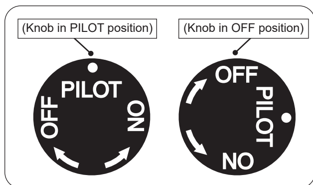
Fig. 45-2 Manual shut down
