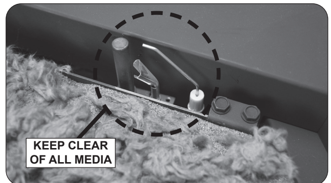
Fig. 19-4 Glowing embers placement detail
