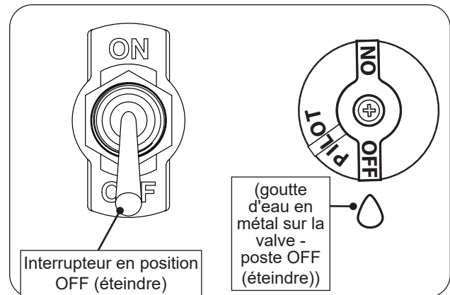
Fig. 70-2 Manual shut down
