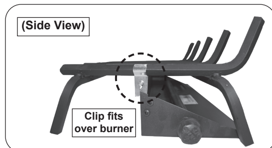
Fig. 11-3 Grate placement detail
