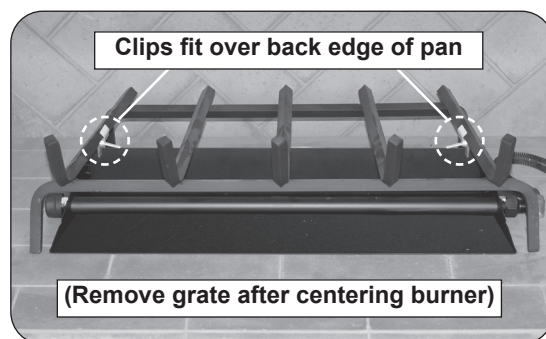
Fig. 11-2 Position grate
