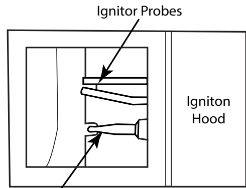
Thermocouple Fig. 6 Proper alignment of probes and thermocouple.
