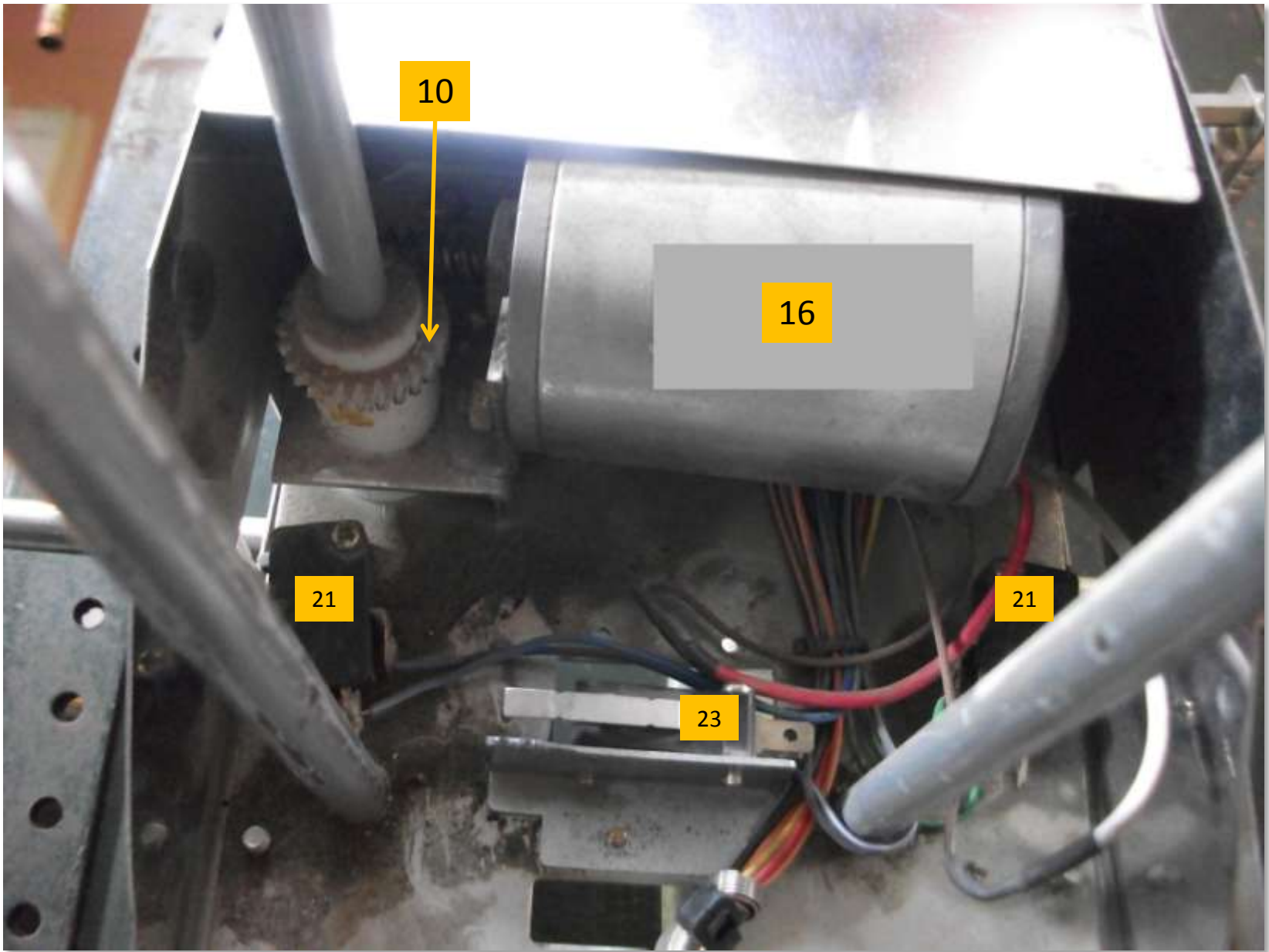
TAIWAN GANTRY Left Side End Plate
