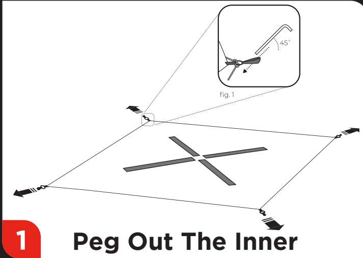
Inner Tent
