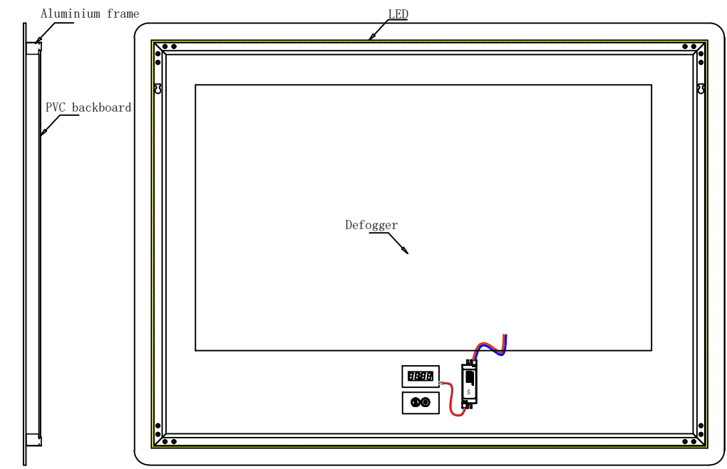
Side View
