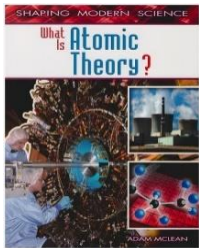
What is Atomic Theory?
