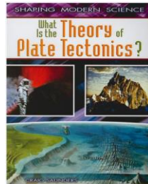
What is the Theory of Plate Tectonics?
